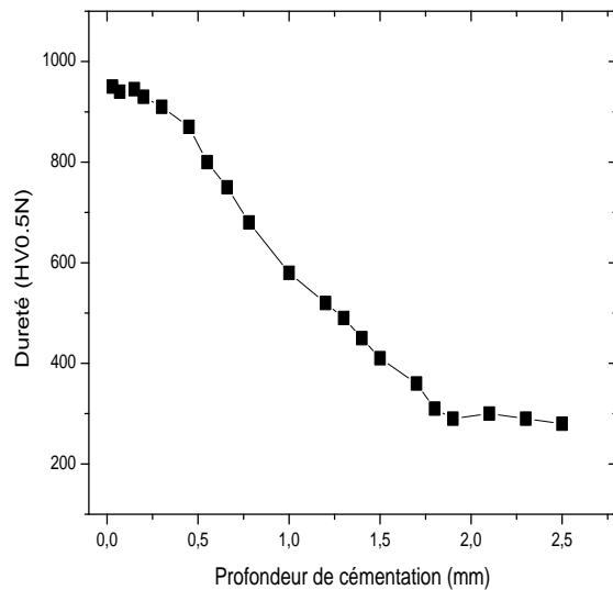
Figure 5: Hardness of Steel Carburized at 830°C for Time of 2h
