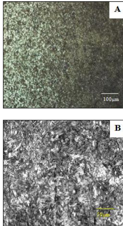
Figure 1: Micrograph of A) Surface Zone and B) Inner Area of the Steel
