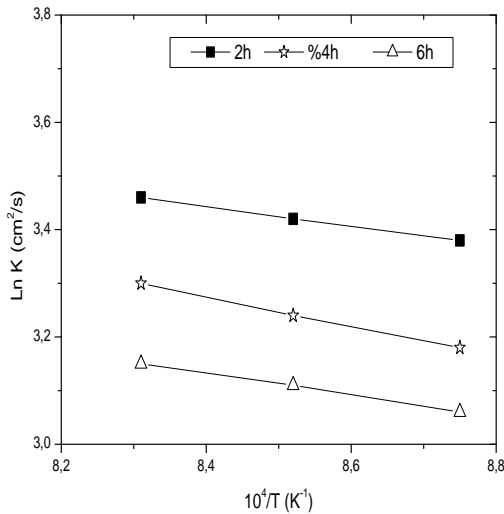
Figure 4: Growth rate constant versus temperature of carburized steel 20CM4
