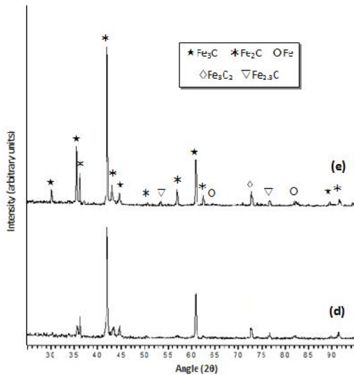
Figure 3: Diffraction Spectra of Steel Carburized at 930°C for 4h (d), 6h (e).
