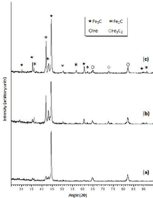
Figure 2: Diffraction Spectra of Steel Carburized for 2h at 870°C (a), 900 °C (b), 930 °C (c)
